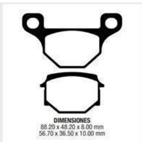
PASTILLA5** JGO PASTILLA FRENO SUZUKI GN 125 / CUSTOM 125 / CUSTOM 200/SKUA 250
