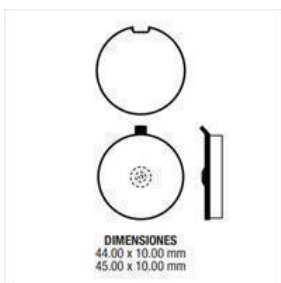
PASTILLA8** JGO PASTILLA FRENO DAKAR 200/TUNDRA/SKUA 150
